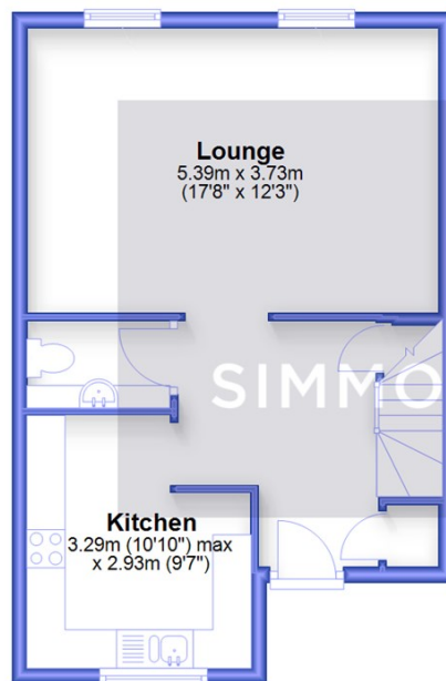
Split Level First Floor
